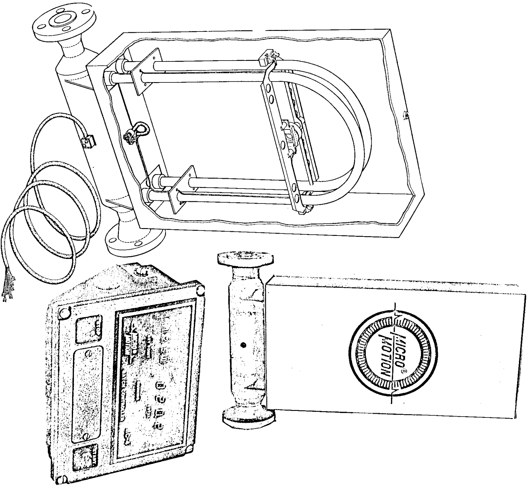
SENSOR UNIT CUTAWAY DRAWING
