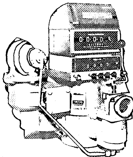
T-11 meter equipped with T2A air eliminator, SP2 set stop faucet, push button set stop counter and counter-printer combination.
