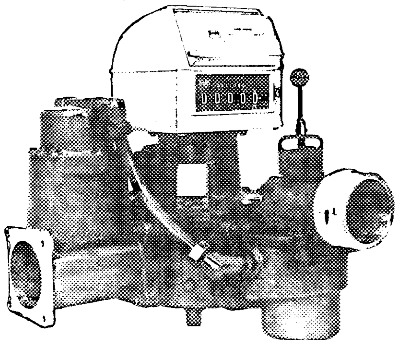
T-40 Meter with Air Eliminator and Faucet
