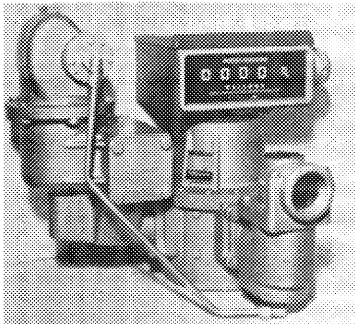
T-11 meter equipped with T2A air eliminator, CP2 faucet and large numeral counter.
