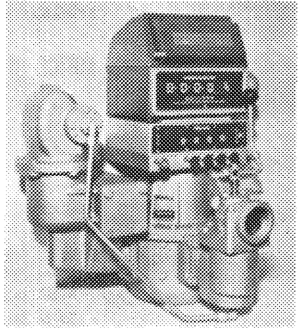
T-11 meter equipped with T2A air eliminator, SP2 set stop faucet, push button set stop counter and counter-printer combination.
