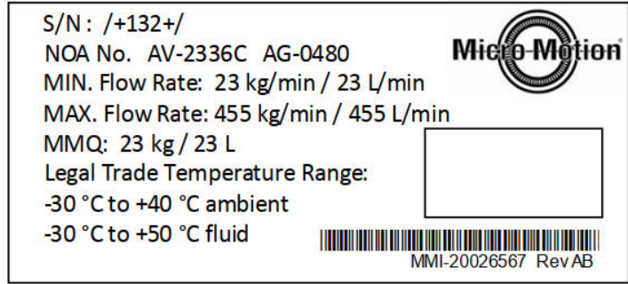
Figure 15 Approval nameplate (CMF100) | La plaque signalétique d’approbation (CMF100)
