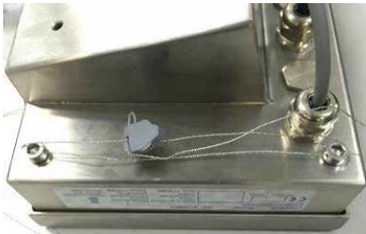
Typical Sealing / Scellage typique
