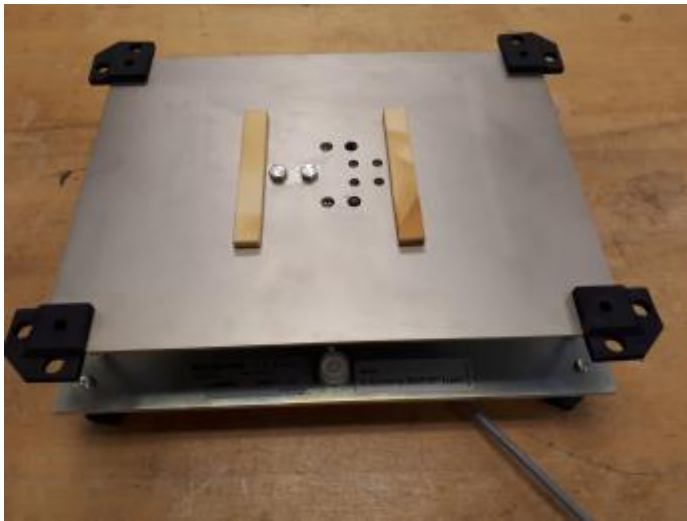
Typical SP4M C6 MR 15 kg, PC 6 C3 20 kg Y=12500 and SP4M C3 MR 30 kg Sub-platter / Sous-plateaux SP4M C6 MR 15 kg, PC 6 C3 20 kg Y=12500 et SP4M C3 MR 30 kg typiques
