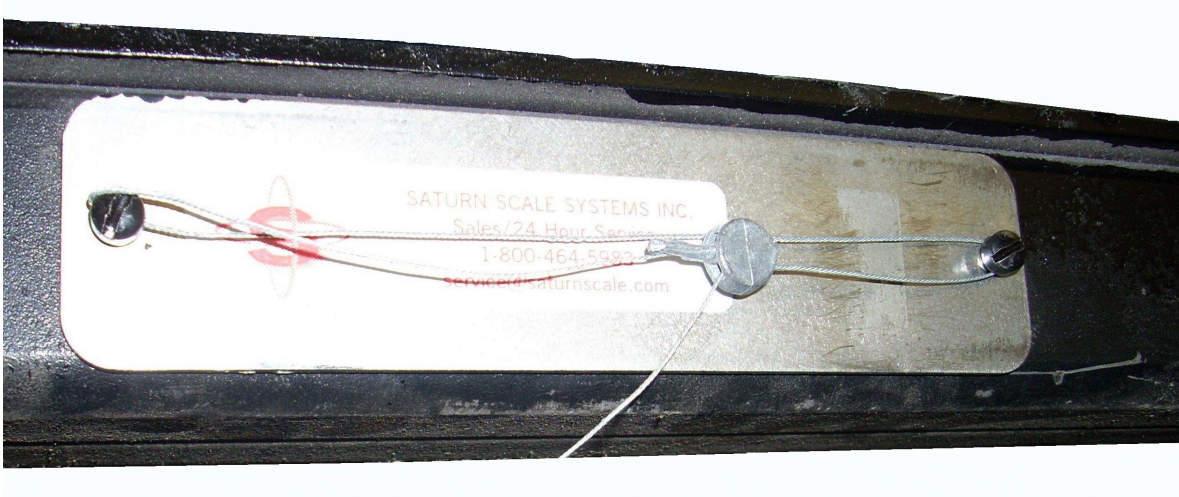
Typical sealing / Scellage typique
