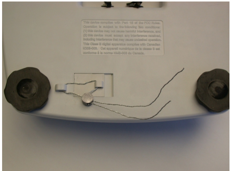
Typical V51P* sealing / scellage typique du V51P*
