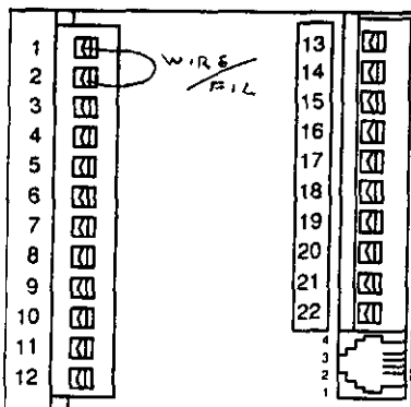
TERMINAL BLOCK Bornier
