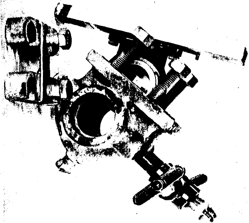
ROBINSON "ORIFICEMASTER" ORIFICE FITTING
