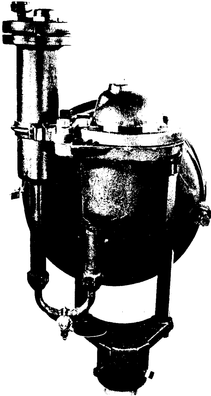
FOXBORO TYPE "28" ORIFICE FLOW METER (Rear View of Differential Element)
