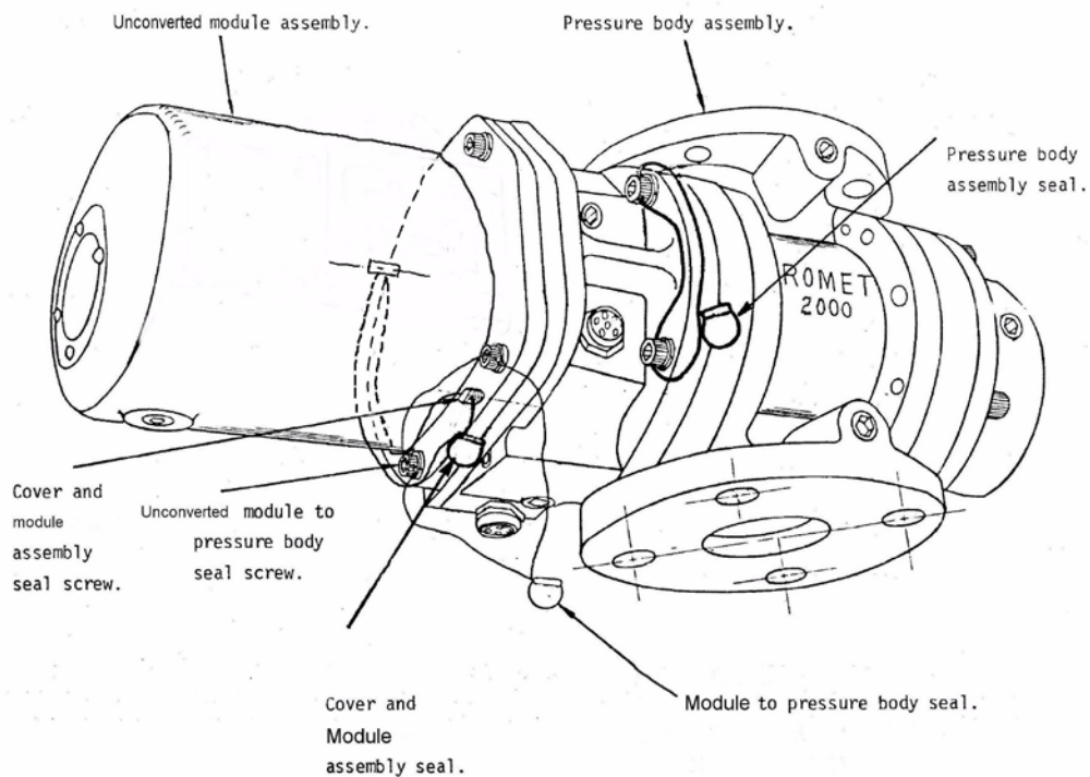
Fig. 6: Sealing / Scellage
