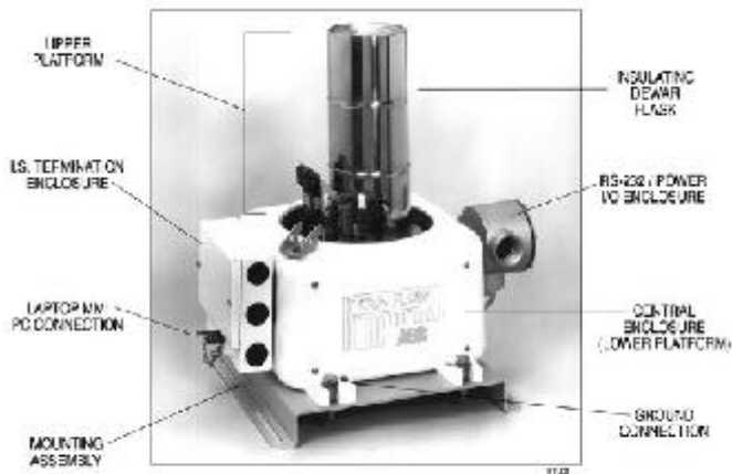
Figure 1-1. Btu/CV Transmitter without Bell Housing
