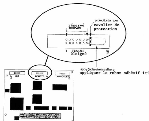
Figure 1. Sealing Arrangement/Installation de plombage
