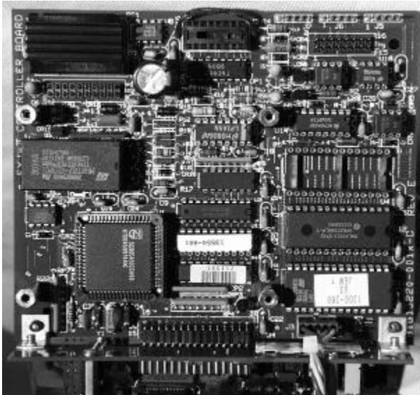
Demand Register EPROM Location on EXJ Register Board (with Display)
