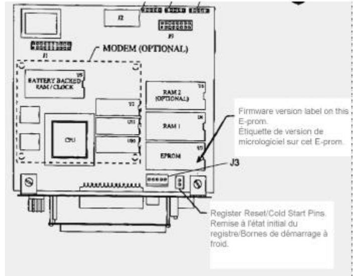
Demand Register EPROM Location on EXJ Register Board (with Display)
