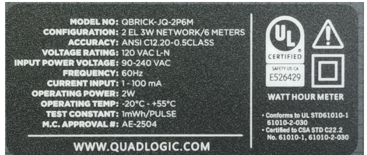
Figure 10 – Nameplate / plaque signalétique
