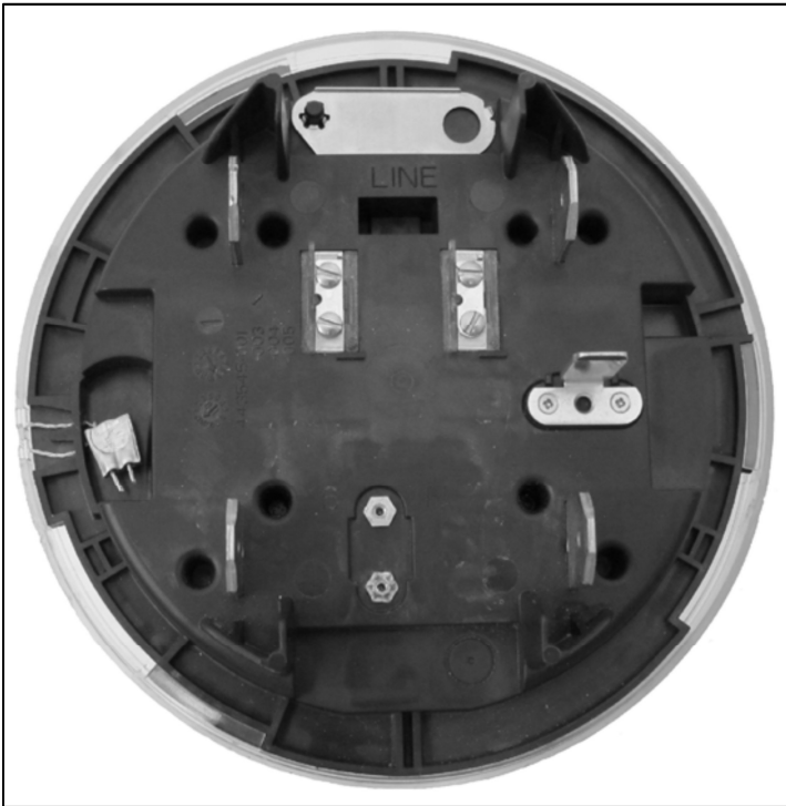
Sealing / Scellage
