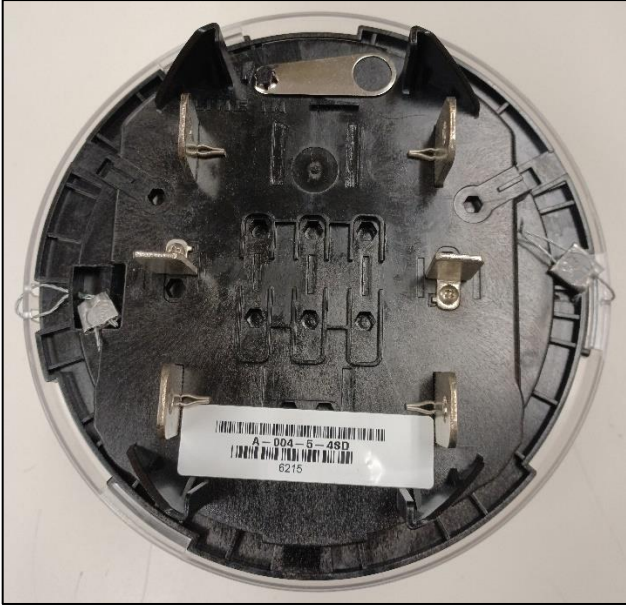
Sealing/ Scellage
