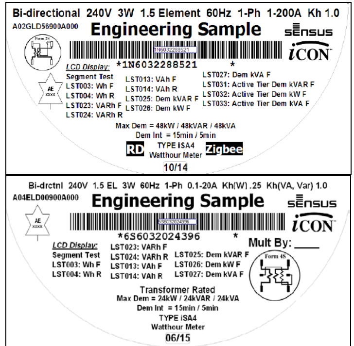
iSA4 Nameplates / Plaques signalétiques iSA4
