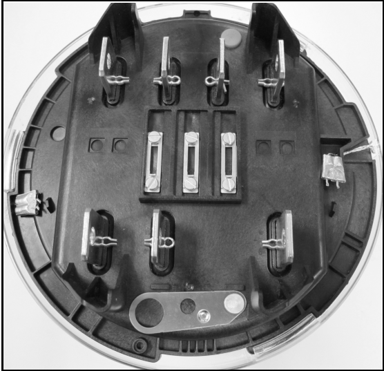
GE kv2c sealing/GE kv2c scellage
