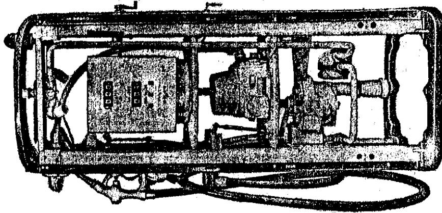
Turbine Pump
