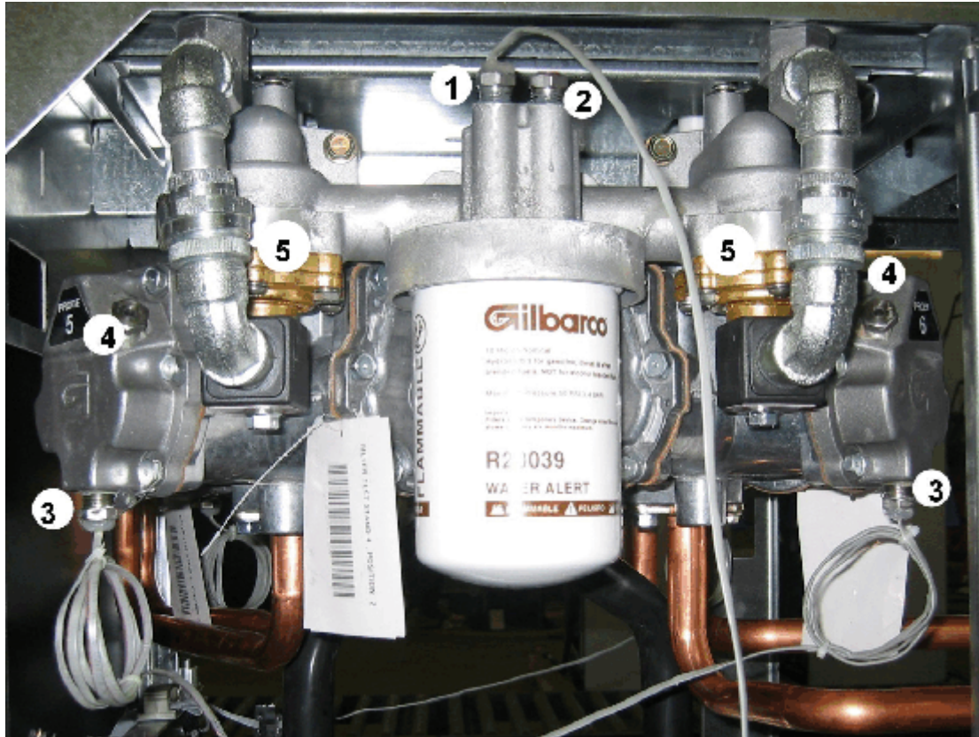
Skinner Valves with Manifold
