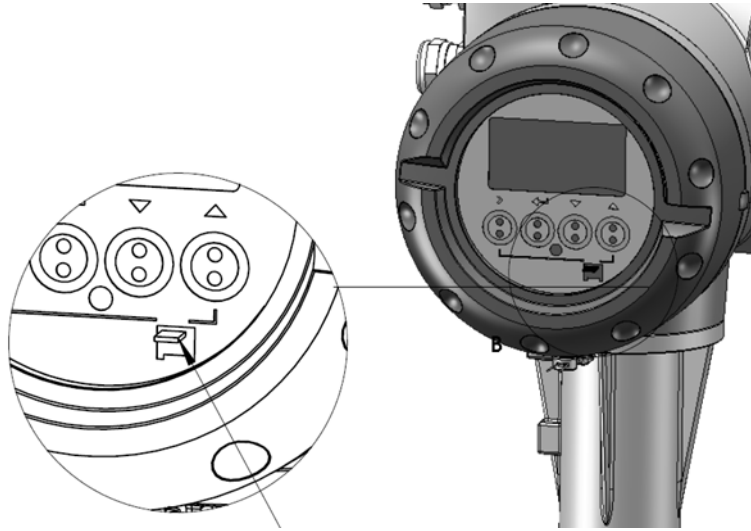
Figure 1. CT Lock Jumper on LCI 40| Cavalier de verrouillage CT du LCI 40
