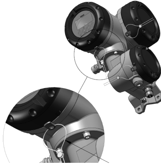
Figure 2: Sealing of the three caps on the LCI 40 Scellage des trois couvercles du LCI 40
