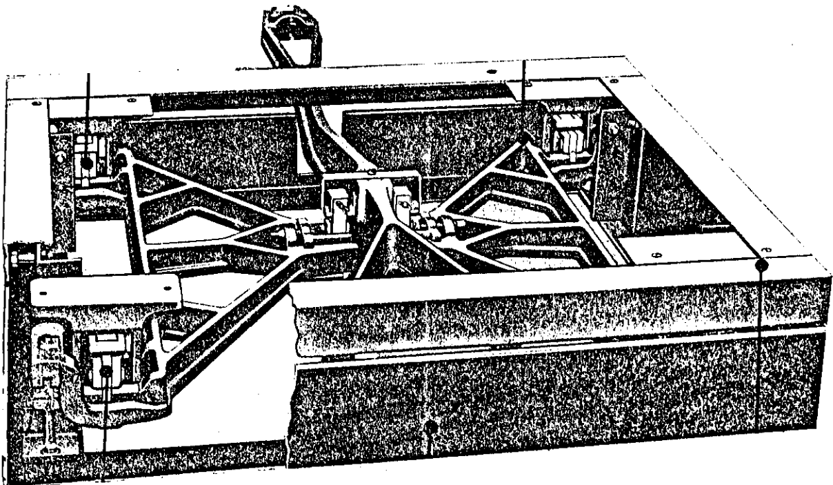
Type "S" lever System
