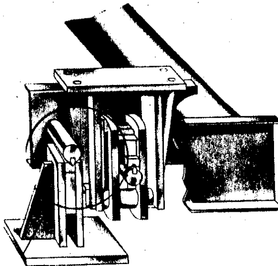
PARALLEL LINK LOAD SUSPENSION ASSEMBLY
