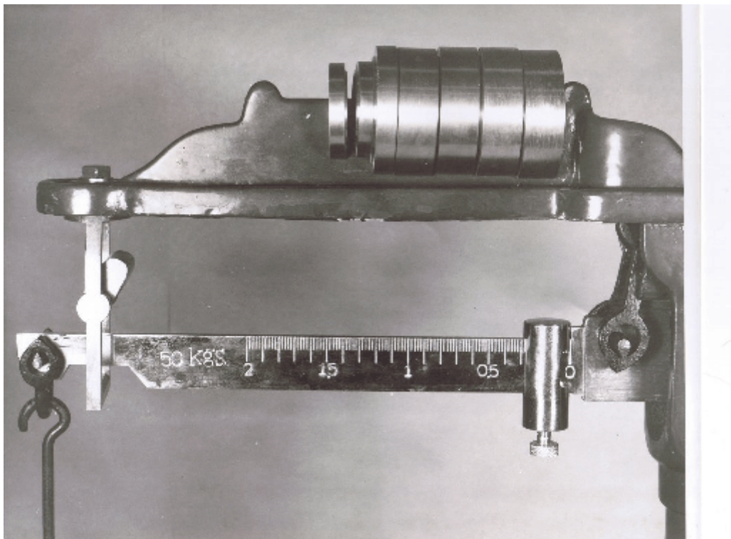
Typical beam and poise assembly on Model SP901/Fléau et contrepoids du modèle SP901
