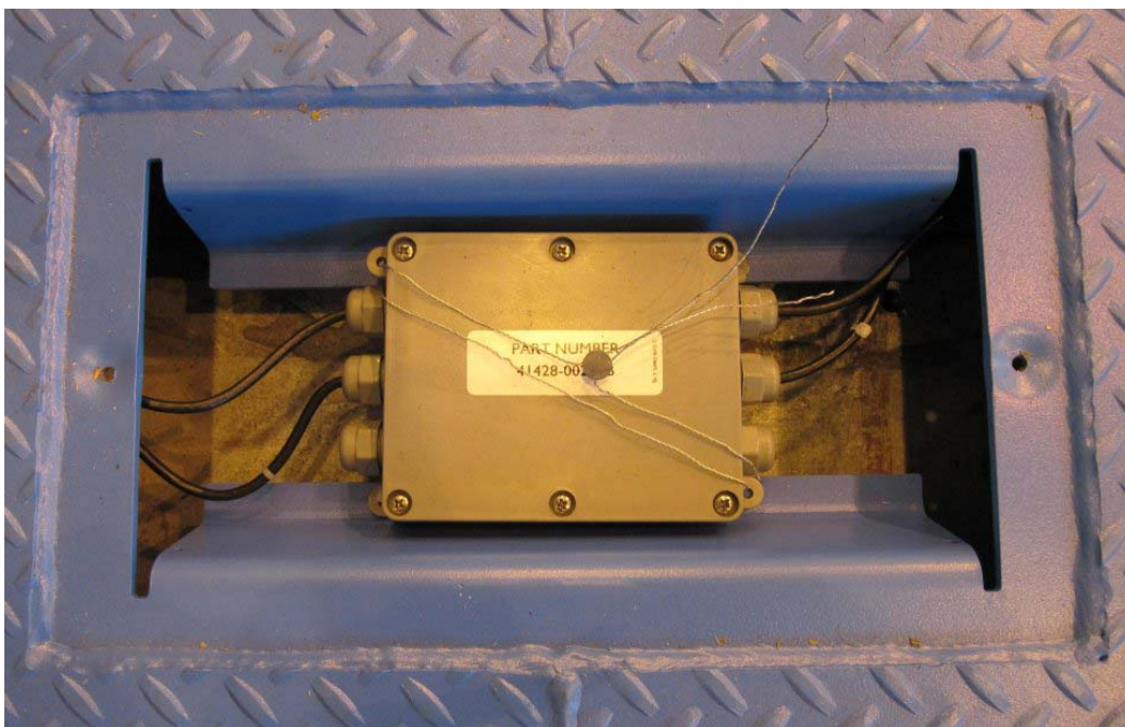
Sealing / Scellage
