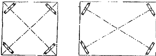
Typical mounting, 3 or 4 load cells Montage type 3 ou 4 cellules de pesage
