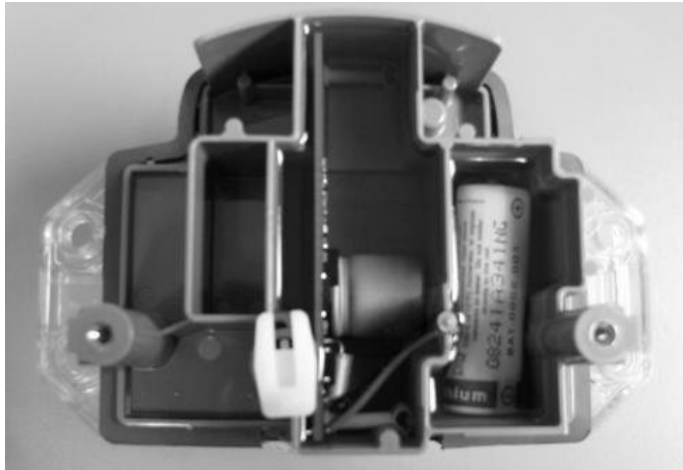
Fig. 13: 100G Datalogging ERT, Part No. ERG-5002-001 (Front View)
