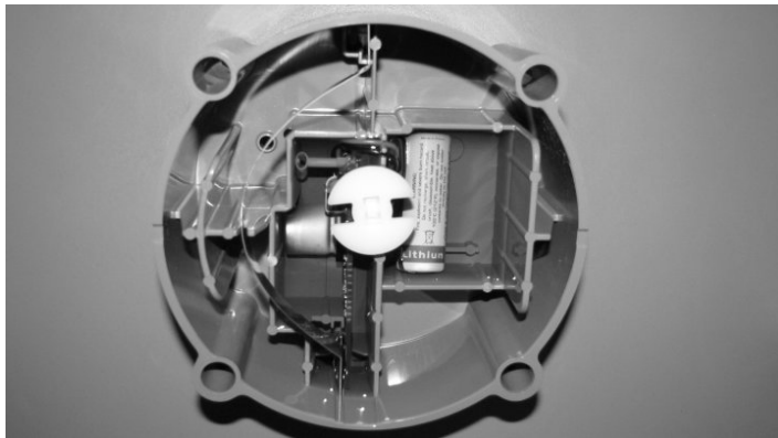
Fig. 15: 100G Datalogging ERT, Part No. ERG-5002-007 (Front View)
