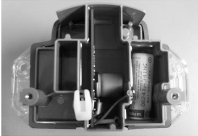
Fig. 13: 100G Datalogging ERT, Part No. ERG-5002-001 (Front View)
