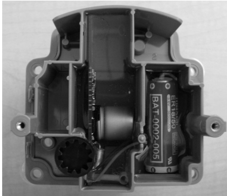
Fig. 17: 100G Datalogging ERT, Part No. ERG-5002-002 (Front View)
