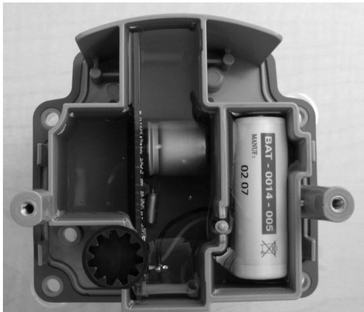
Fig. 16: 100G ERT, Part No. ERG-5000-002 (Front View)
