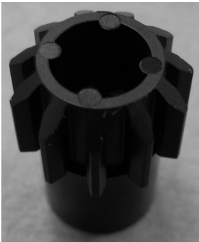
Fig. 19: 11 teeth for ERG-5000-002 and ERG-5002-002 / 11 dents pour ERG-5000-002 et ERG-5002-002
