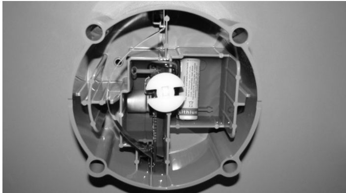
Fig. 15: 100G Datalogging ERT, Part No. ERG-5002-007 (Front View)
