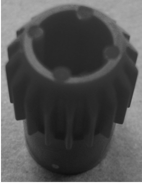
Fig. 21: 18 teeth for ERG-5000-004 and ERG-5002-004 / 18 dents pour ERG-5000-004 et ERG-5002-004
