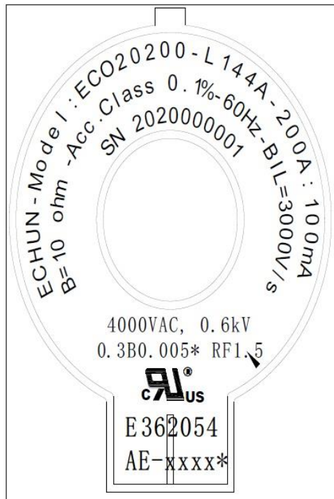
Figure 2 – Nameplate / Plaque signalétique
