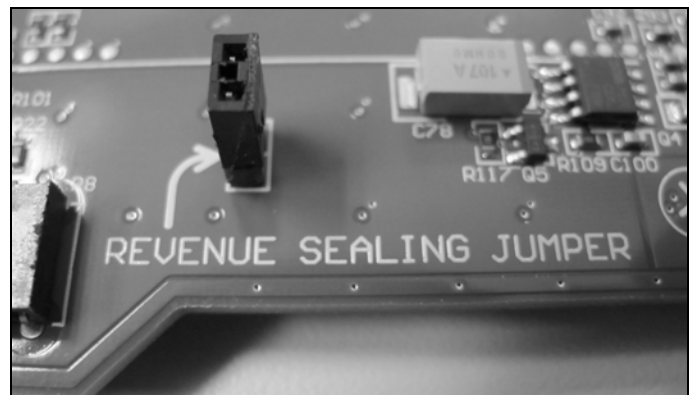
Revenue Sealing Jumper / Bretelle de scellage de revenu
