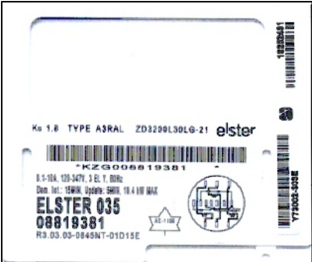
Aclara UMT-C-A3 markings/marquages
