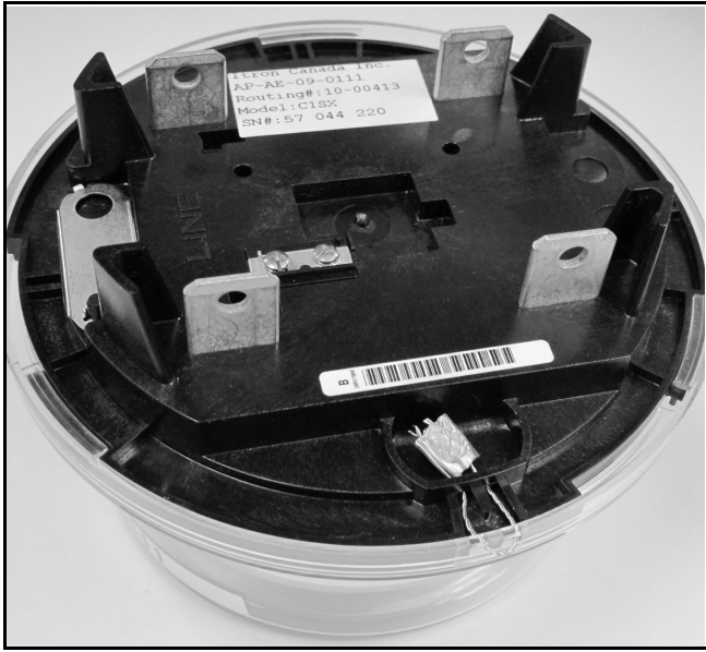
Itron C1SX sealing / Itron C1SX scellage
